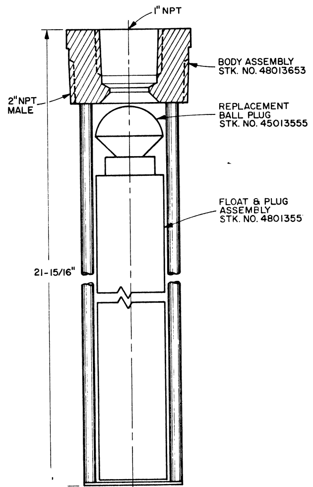
Model 80 Gas Scrubber Valve
